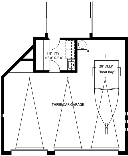
OPTIONAL THREE CAR GARAGE
